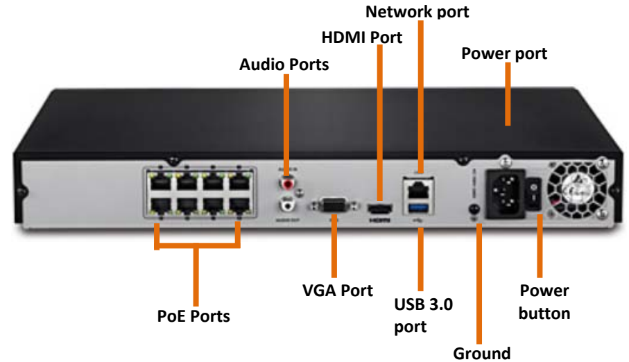
Rear View
