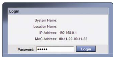
Figure 14. Login
