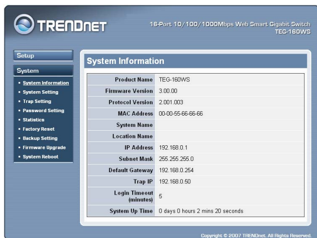
Figure 15. System Information
