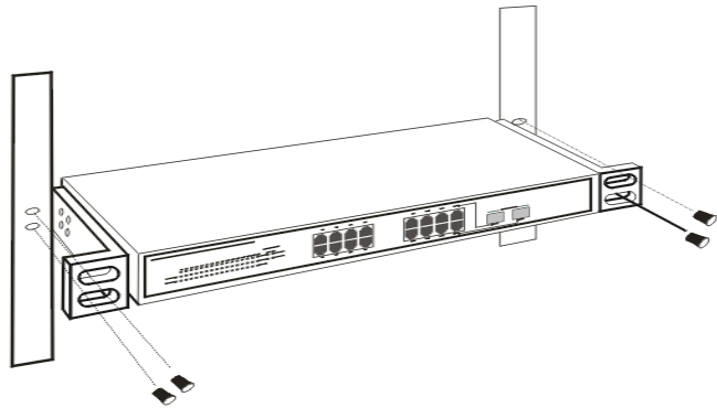
Figure 3. Mount the Switch in the rack
