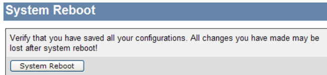
Figure 36. System Reboot
