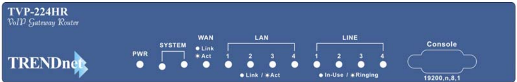
4-port TVP-224HR Front Panel
