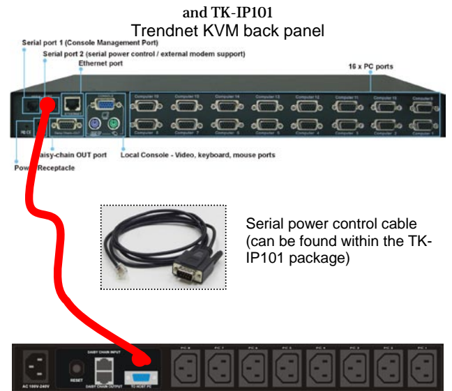
TK-RP08 Backpanel
