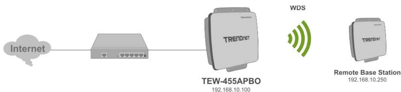
Figure 4-1 Point to Point Configuration
