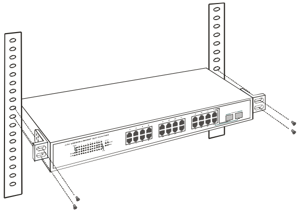
Figure 3. Mount the Switch in the rack
